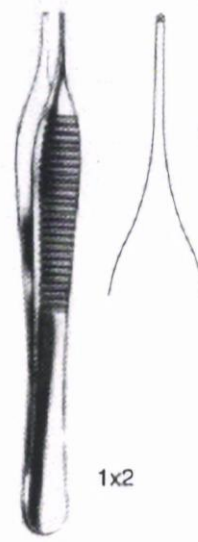
ADSON micro 11186-12 12,0 cm 11186-15 15,0 cm
